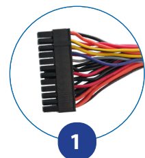
1 M/B 20+4P 1pc / 500mm
